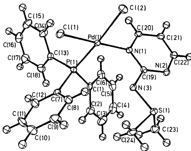
Figure 2. A view of cis - [\text{PdCl}_2(\text{PPh}_3)(\text{Me}_2\text{SNC}_4\text{H}_3\text{N}_2)] ( 4f ), showing 50% probability ellipsoids
