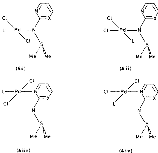
Figure 1. Isomeric forms of [\text{PdCl}_2\text{L}(\text{Me}_2\text{SNR})] ( 4 ) ( \text{L} = tertiary phosphine, \text{R} = 2-pyridyl or 2-pyrimidinyl, \text{X} = \text{CH}, \text{N} )
