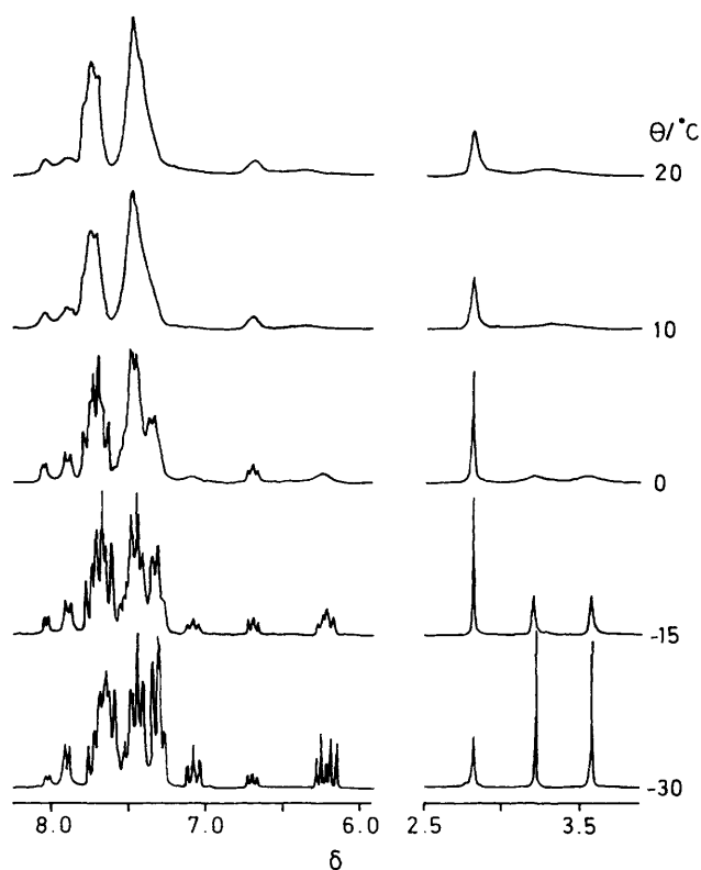
Figure 3. Variable-temperature 1 H n.m.r. spectrum of [PdCl 2 (PPh 3 ) 2 ](Me 2 SNC 5 H 4 N)] ( 4d ) in CD 2 Cl 2
